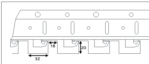
An Overview of the Carrier with 32mm Panels
