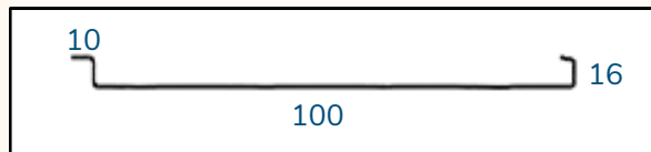
Cross Section of the Ceiling Panels
