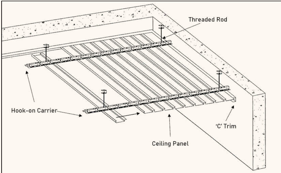
An Overview of the Ceiling System
