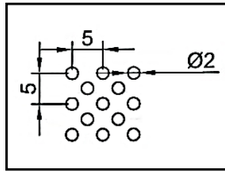
Pattern #20 Open area 22% Centres 5 Staggered Diameter 2.0mm
