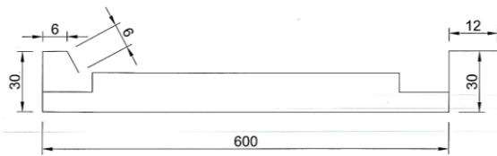
Measurements of the panel
