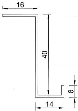
Measurements of the Z-profile
