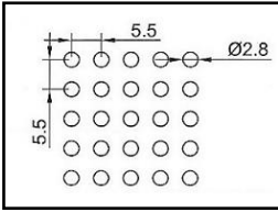
Pattern #28 Open area 20% Centres 5.5 Straight Diameter 2.8mm
