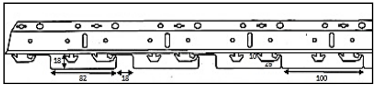
An Overview of Carrier with 100mm panels
