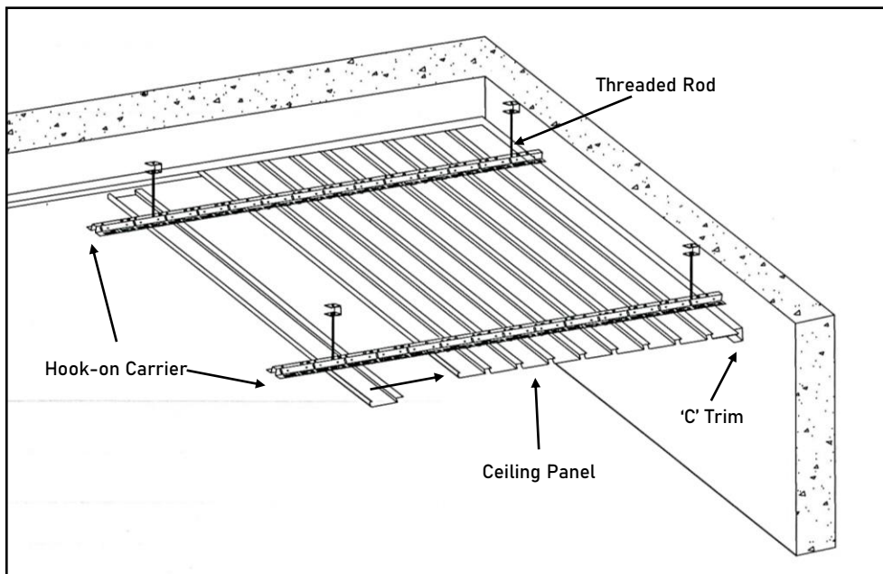
An Overview of the Ceiling System
